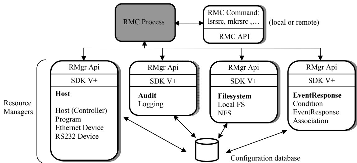
Figure 3: The structure of the RMC subsystem.
